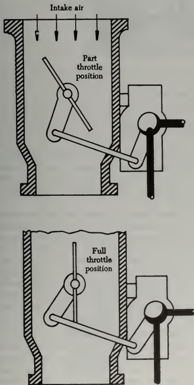
FIGURE 3-36. Fuel/air control unit.
